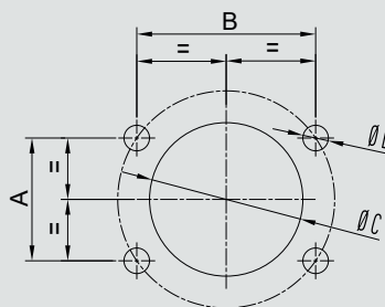
Panel hole pattern
