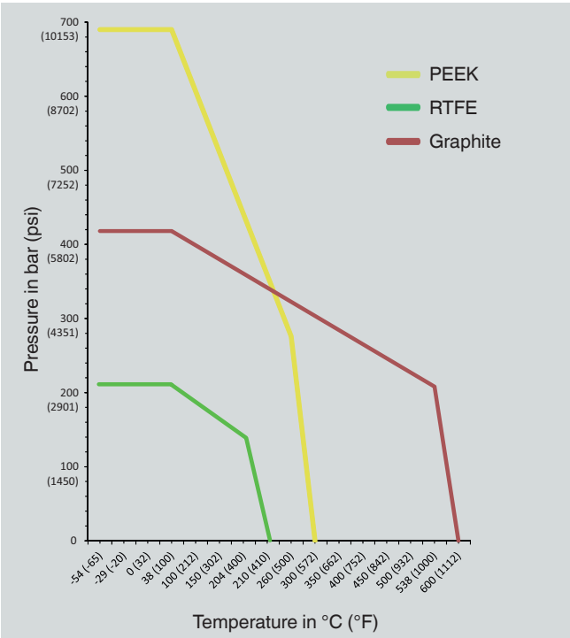
Pressure-temperature diagram
